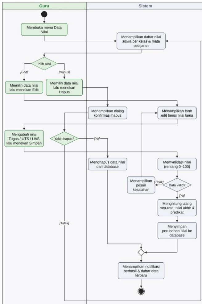
Gambar 9. Activity Diagram Edit / Hapus Nilai
