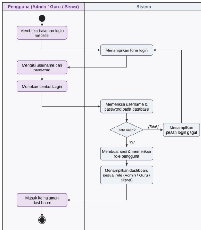
Gambar 1. Activity Diagram Login
