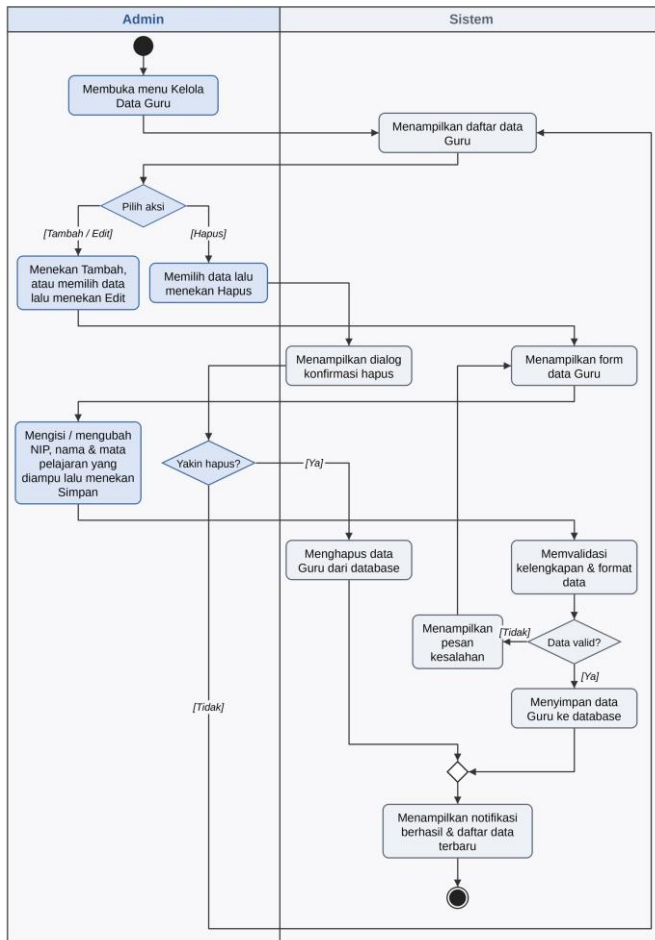
Gambar 3. Activity Diagram Kelola Data Guru
