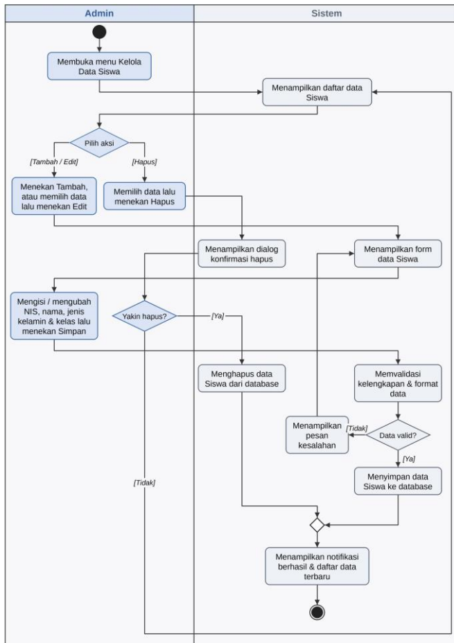
Gambar 4. Activity Diagram Kelola Data Siswa
