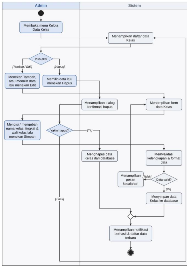
Gambar 5. Activity Diagram Kelola Data Kelas
