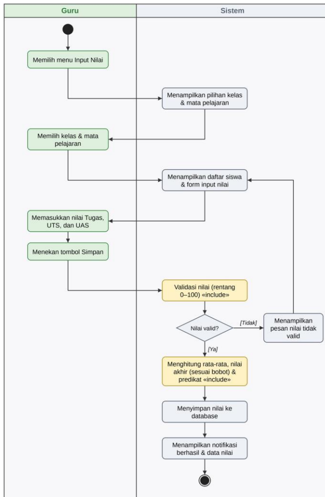
Gambar 8. Activity Diagram Input Nilai (Tugas, UTS, UAS)
