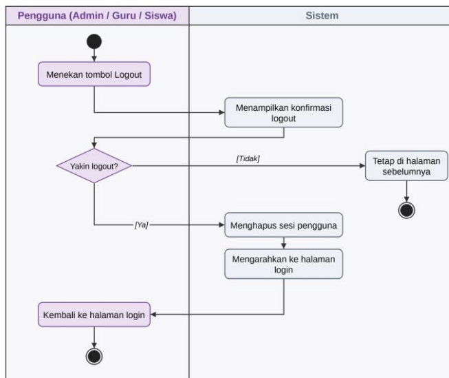
Gambar 12. Activity Diagram Logout
