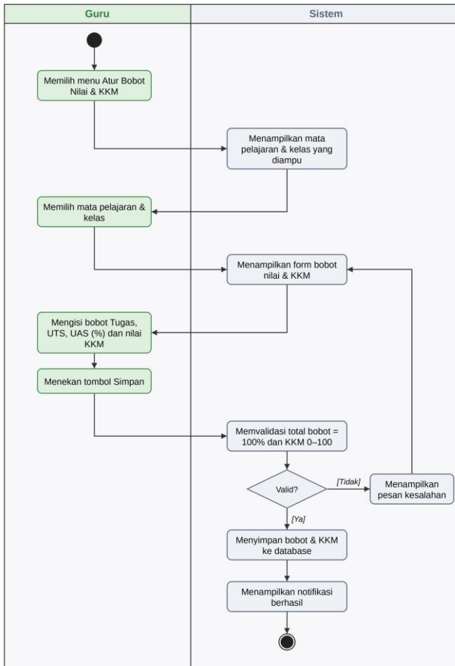
Gambar 7. Activity Diagram Atur Bobot Nilai & KKM
